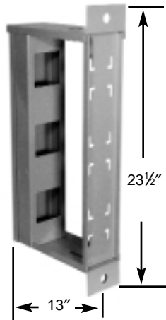
WALL OR POLE MOUNT C.T. RACK S7860
